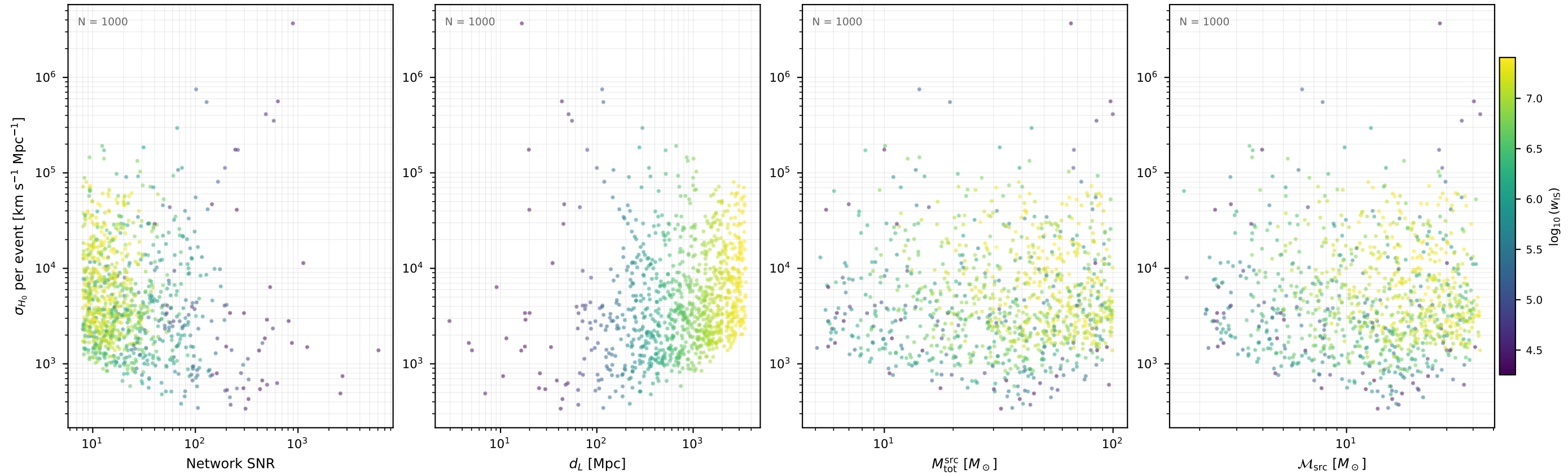
Fisher \sigma_{H_0} per event aLIGO_HLV / baseline (1000 events, 10 seed(s))
