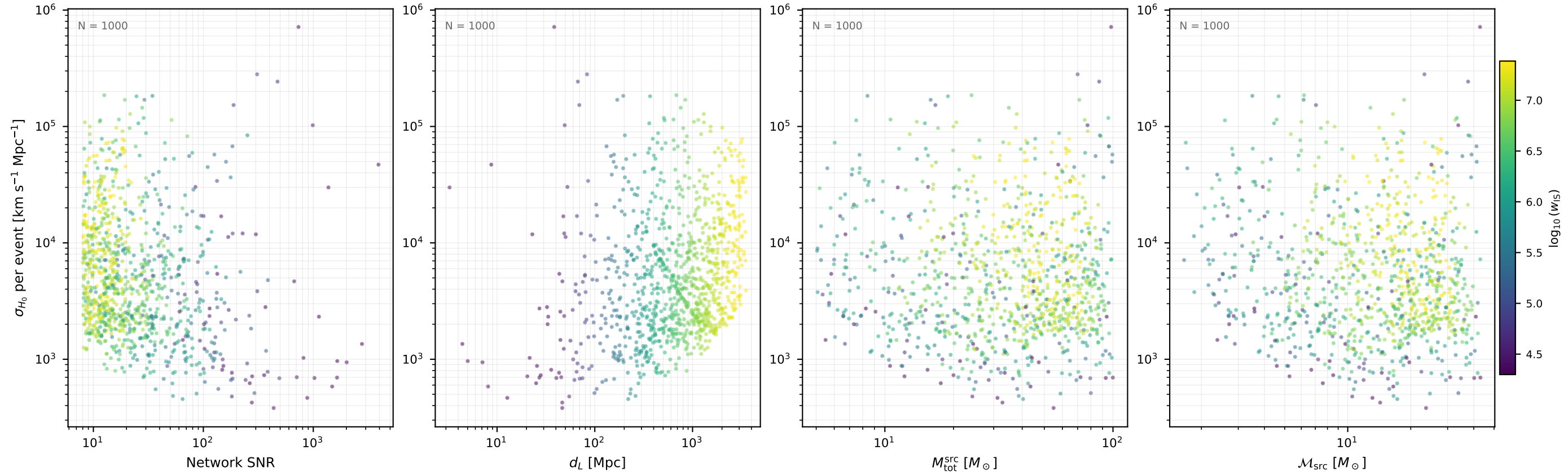
Fisher \sigma_{H_0} per event aLIGO_HLV (1000 events, 10 seed(s))
