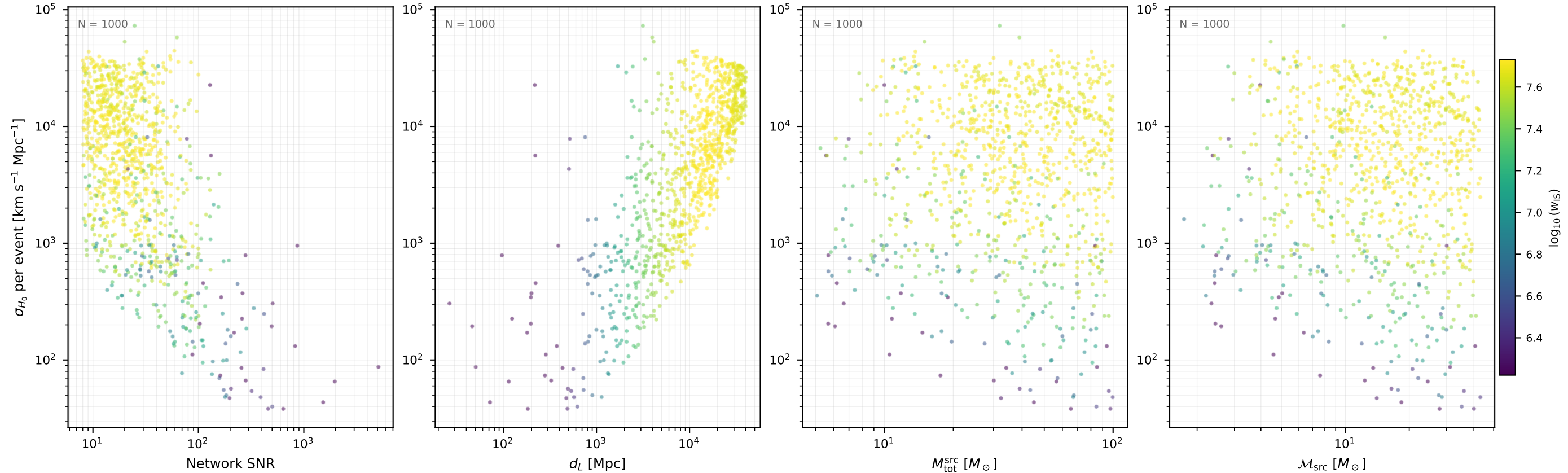
Fisher \sigma_{H_0} per event ET / var01 (1000 events, 10 seed(s))
