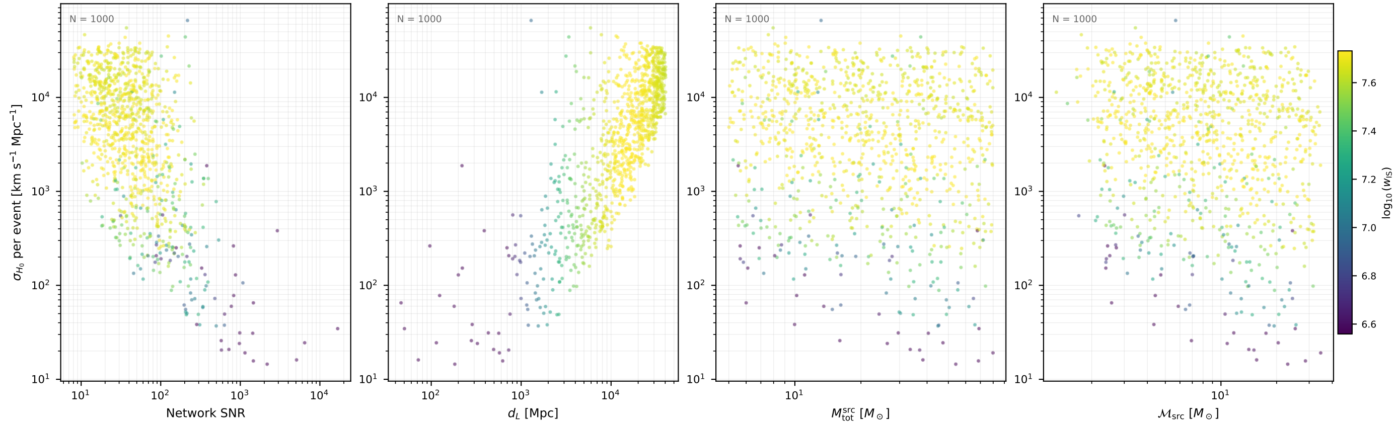
Fisher \sigma_{H_0} per event CE / var06 (1000 events, 10 seed(s))
