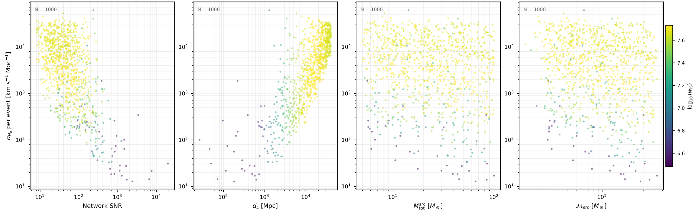
Fisher \sigma_{H_0} per event CE / var03 (1000 events, 10 seed(s))
