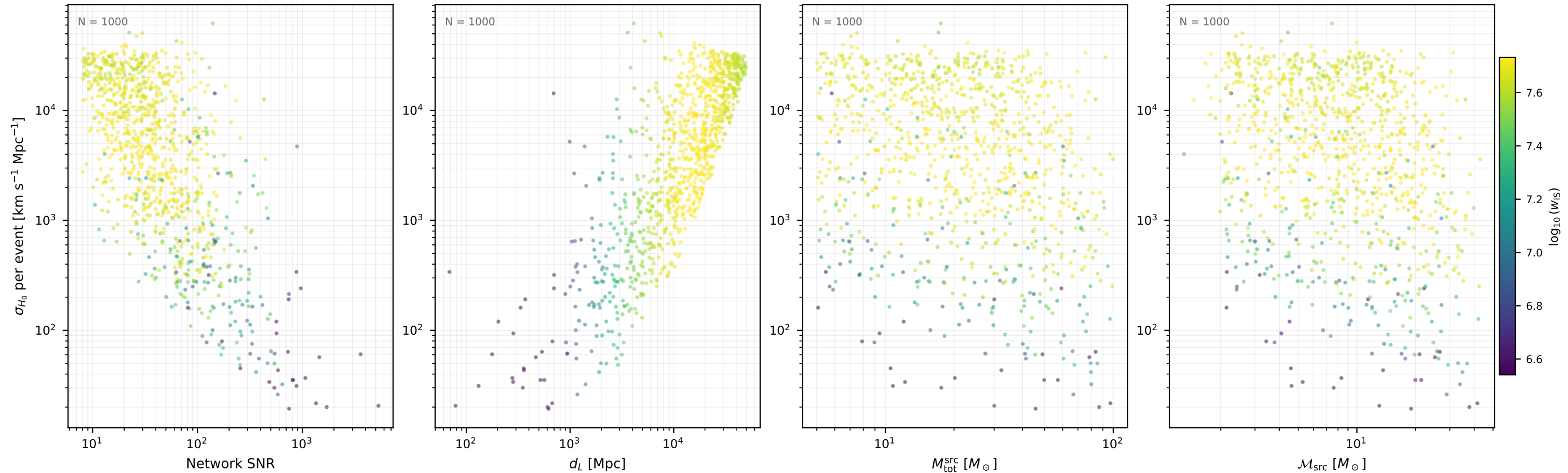
Fisher \sigma_{H_0} per event ET_CE / var04 (1000 events, 10 seed(s))
