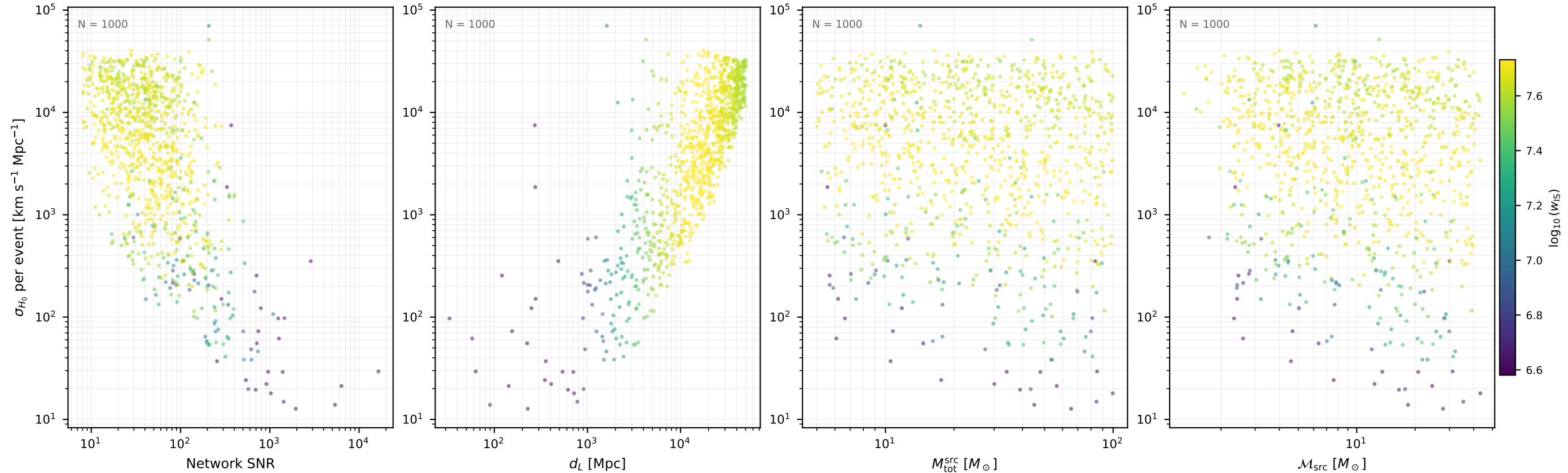
Fisher \sigma_{H_0} per event ET_CE / var03 (1000 events, 10 seed(s))
