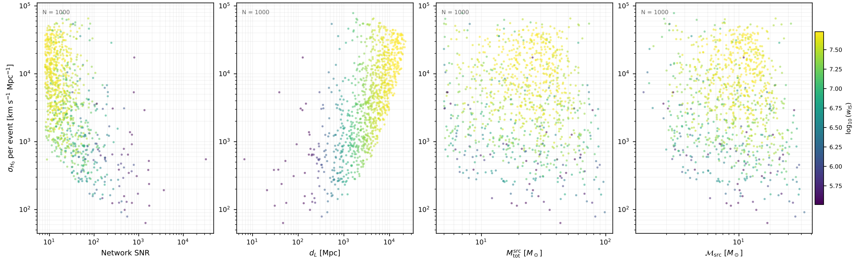
Fisher \sigma_{H_0} per event ET / var05 (1000 events, 10 seed(s))
