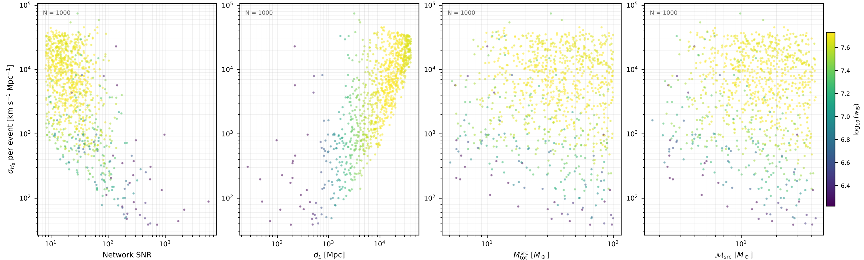
Fisher \sigma_{H_0} per event ET / var03 (1000 events, 10 seed(s))
