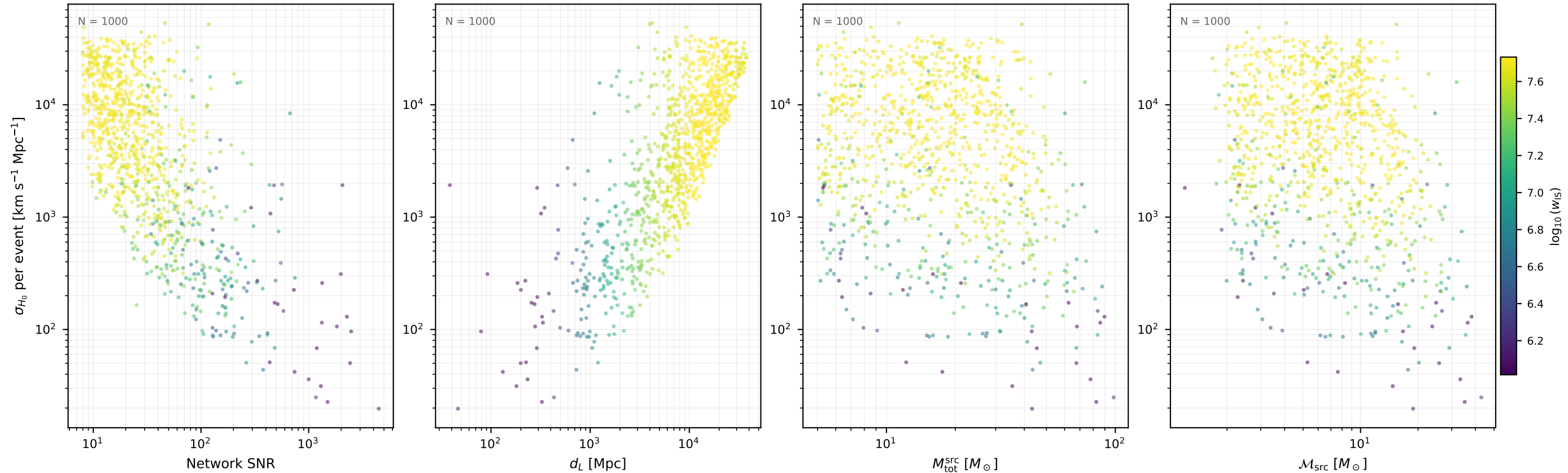
Fisher \sigma_{H_0} per event CE / var05 (1000 events, 10 seed(s))
