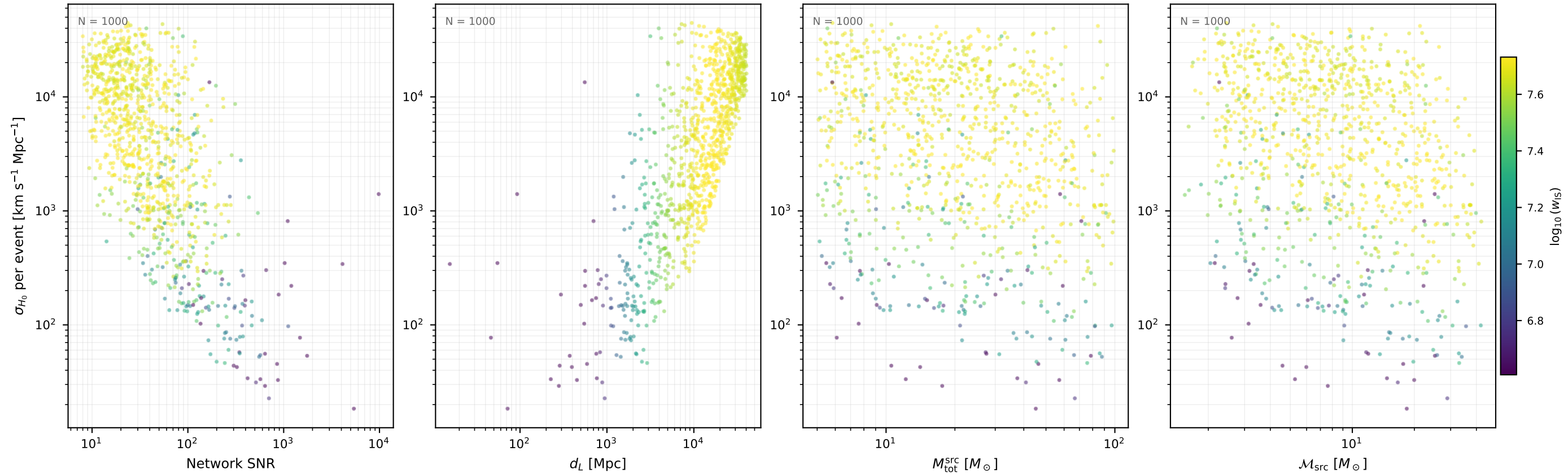
Fisher \sigma_{H_0} per event CE / var04 (1000 events, 10 seed(s))
