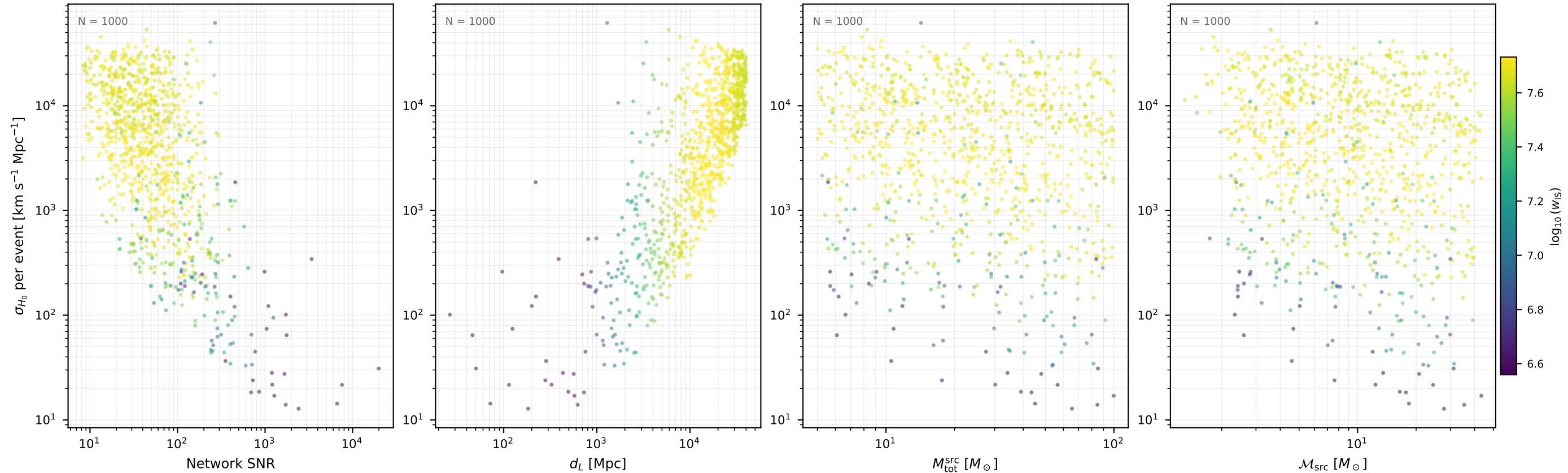
Fisher \sigma_{H_0} per event CE / var02 (1000 events, 10 seed(s))
