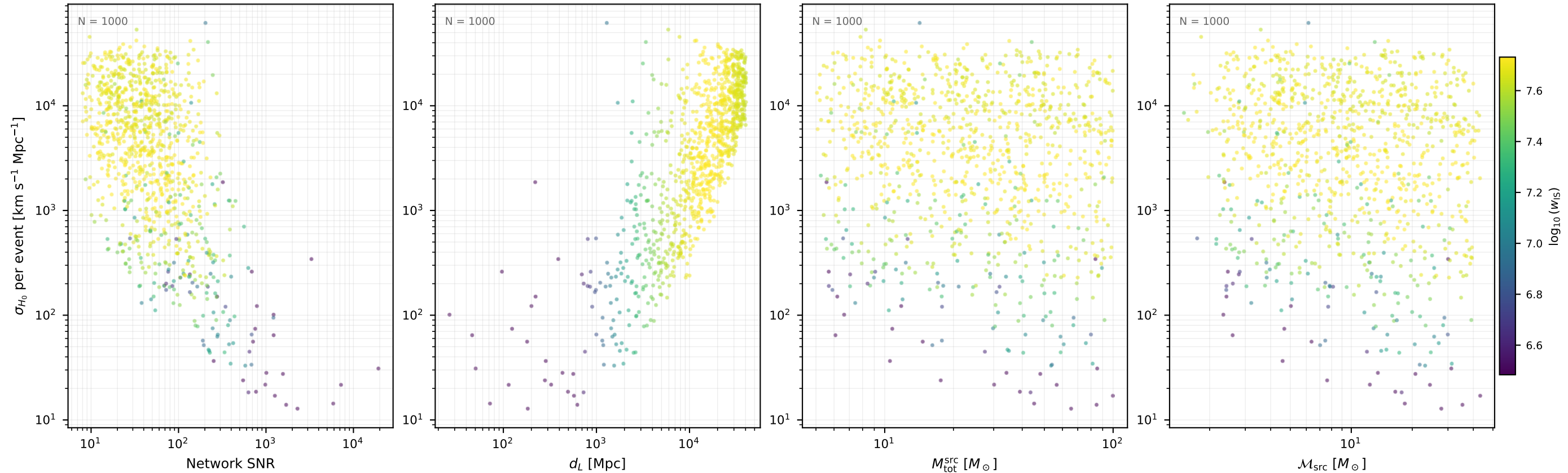
Fisher \sigma_{H_0} per event CE / var01 (1000 events, 10 seed(s))
