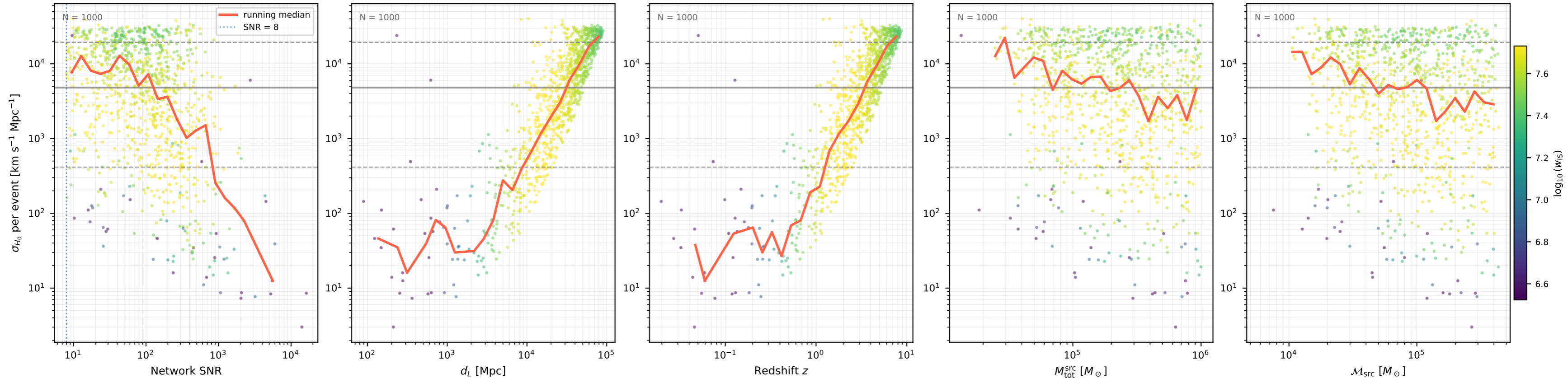
Fisher \sigma_{H_0} per event LISA / light_seeds n_samples=4096 (1000 events, 10 seed(s))
