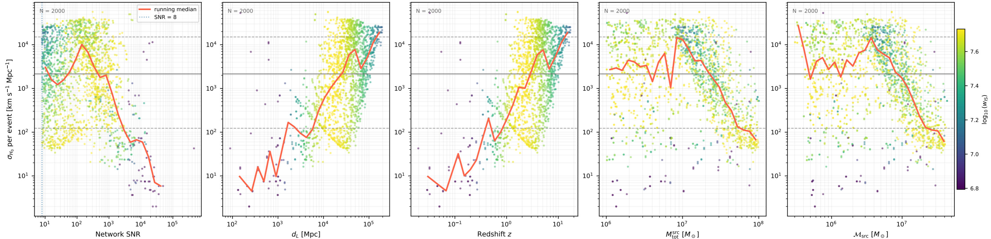
Fisher \sigma_{H_0} per event LISA / heavy_seeds (2000 events, 10 seed(s))
