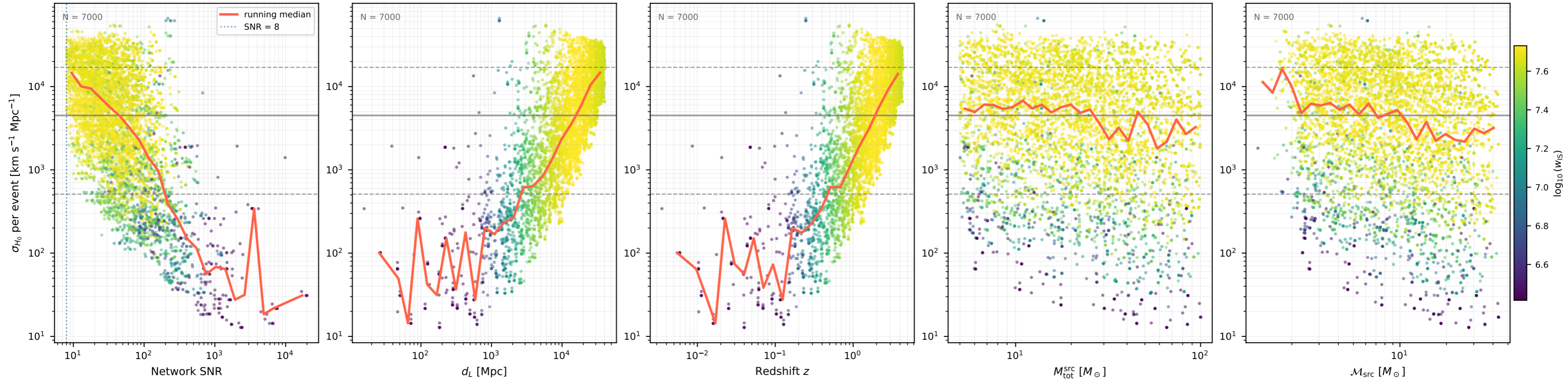
Fisher \sigma_{H_0} per event CE (7000 events, 10 seed(s))
