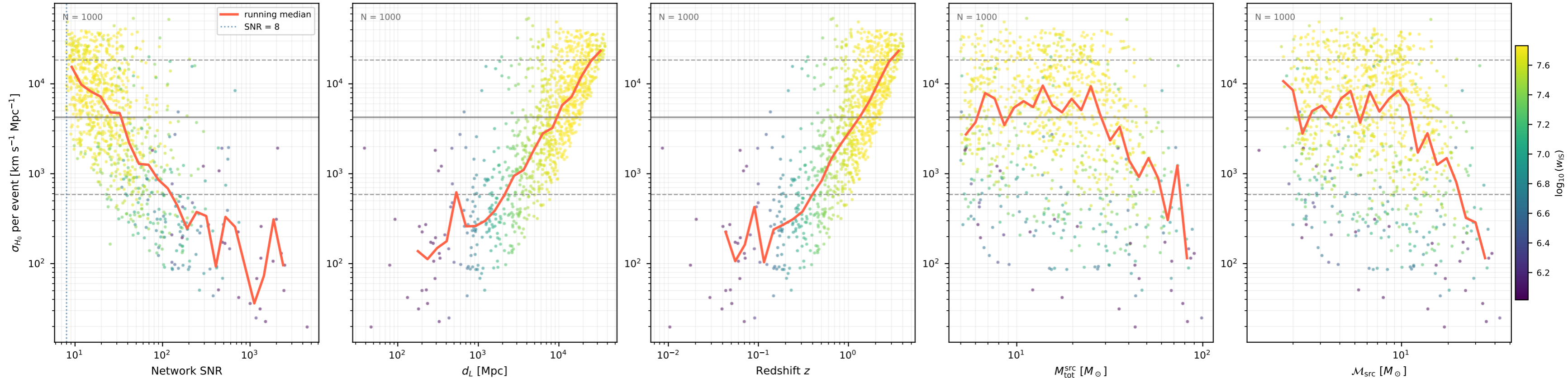
Fisher \sigma_{H_0} per event var05 (1000 events, 10 seed(s))
