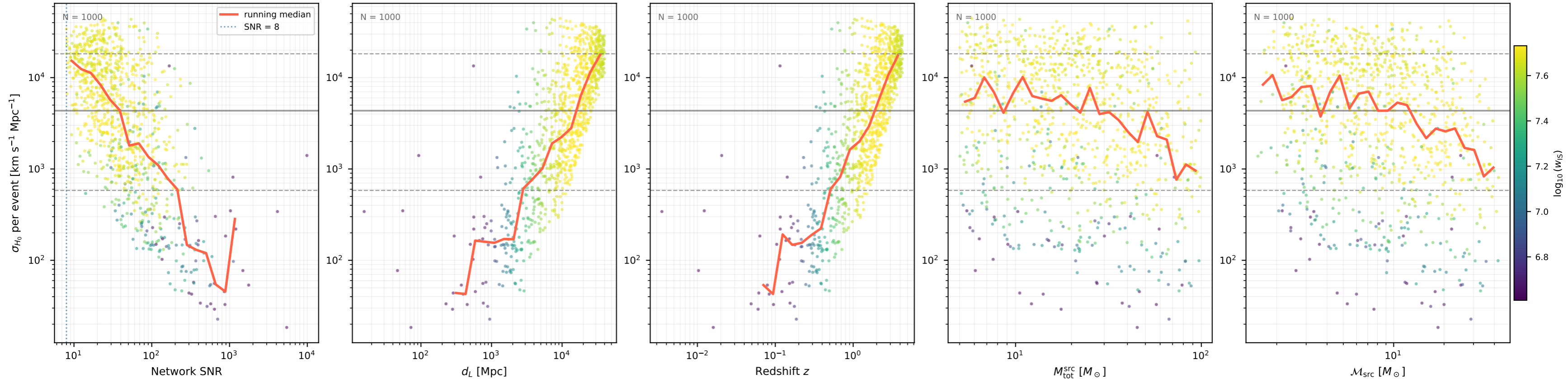
Fisher \sigma_{H_0} per event var04 (1000 events, 10 seed(s))
