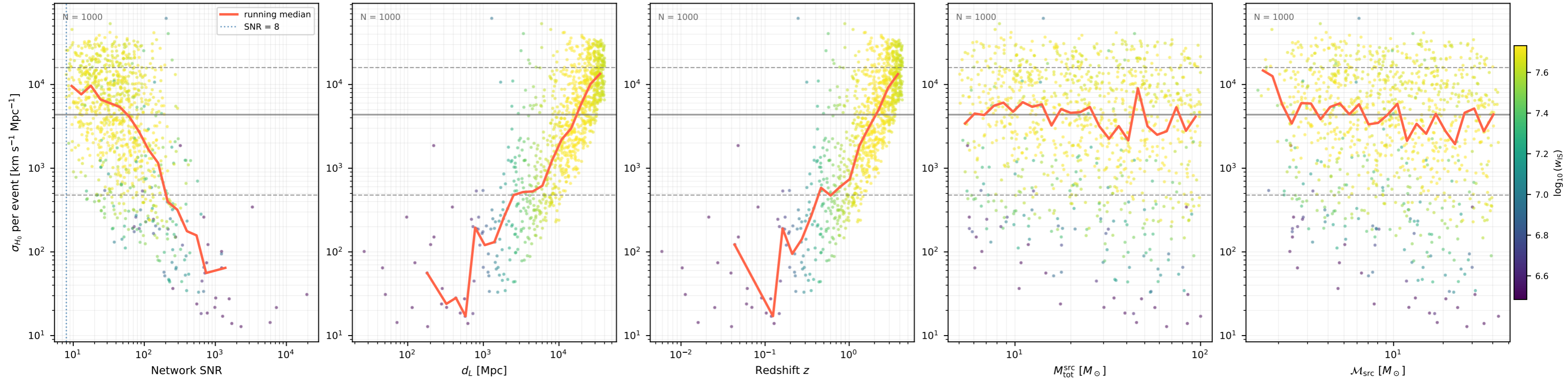
Fisher \sigma_{H_0} per event var01 (1000 events, 10 seed(s))
