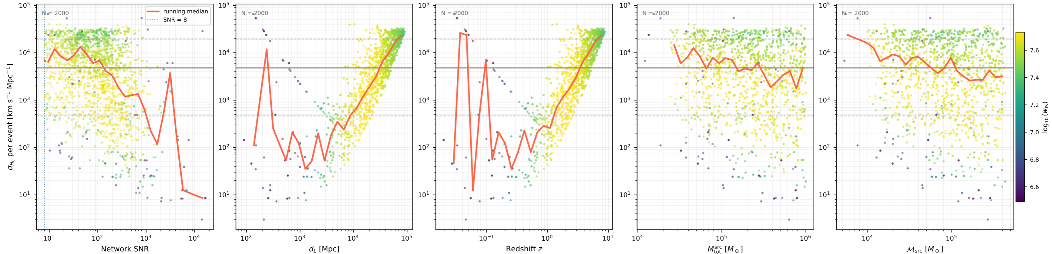
Fisher \sigma_{H_0} per event light_seeds (2000 events, 10 seed(s))
