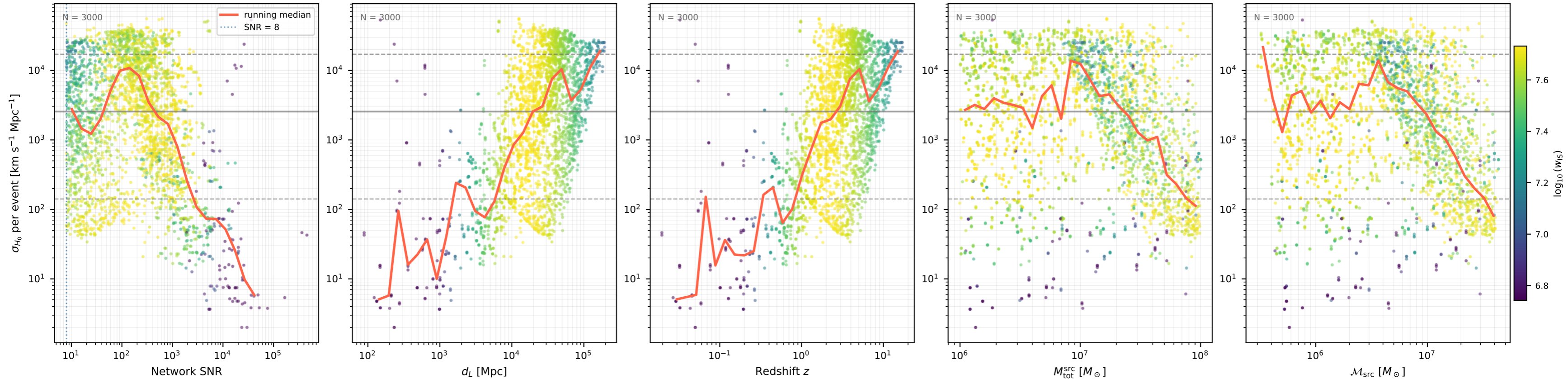
Fisher \sigma_{H_0} per event heavy_seeds (3000 events, 10 seed(s))
