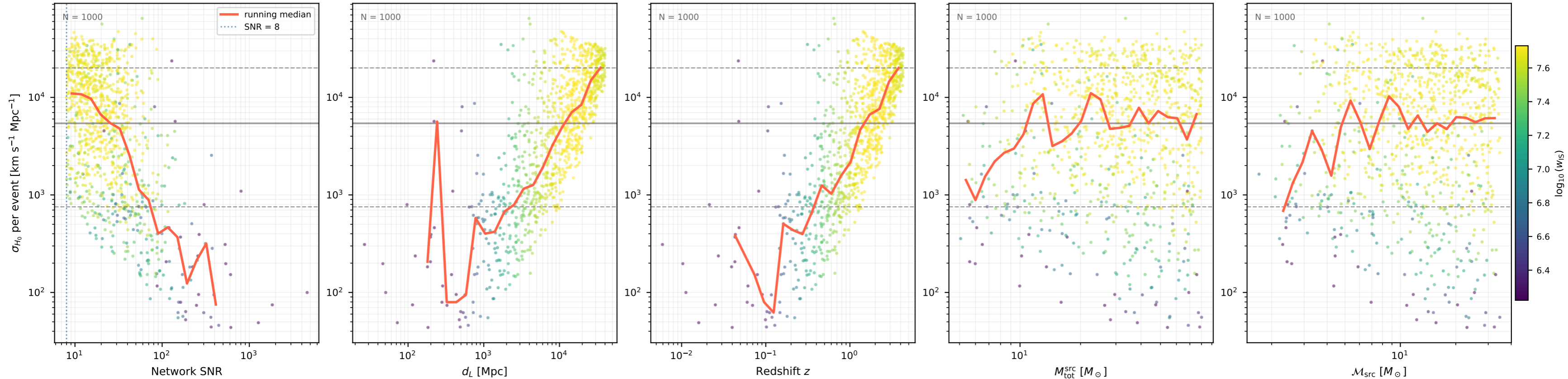
Fisher \sigma_{H_0} per event var06 (1000 events, 10 seed(s))
