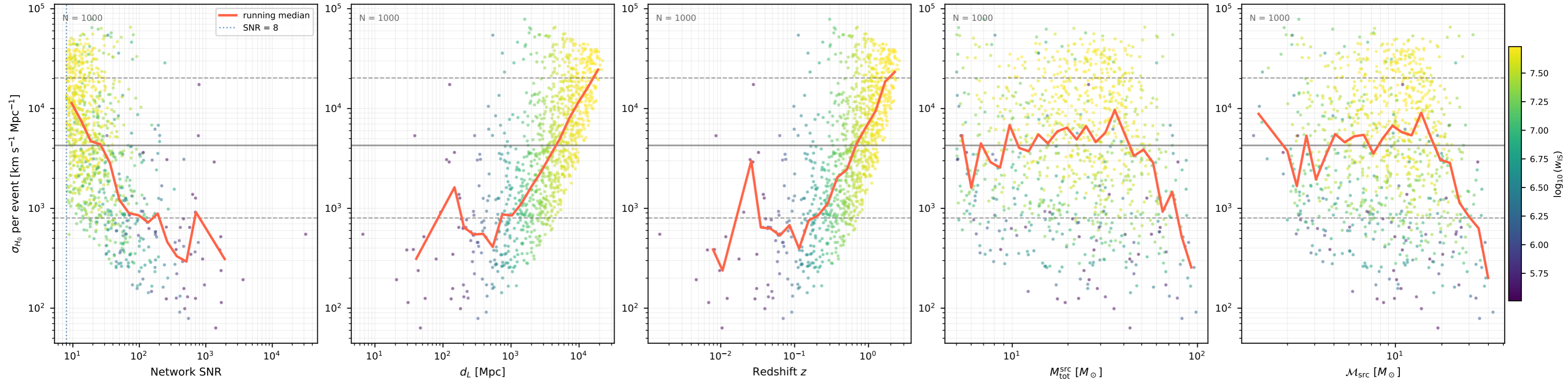
Fisher \sigma_{H_0} per event var05 (1000 events, 10 seed(s))
