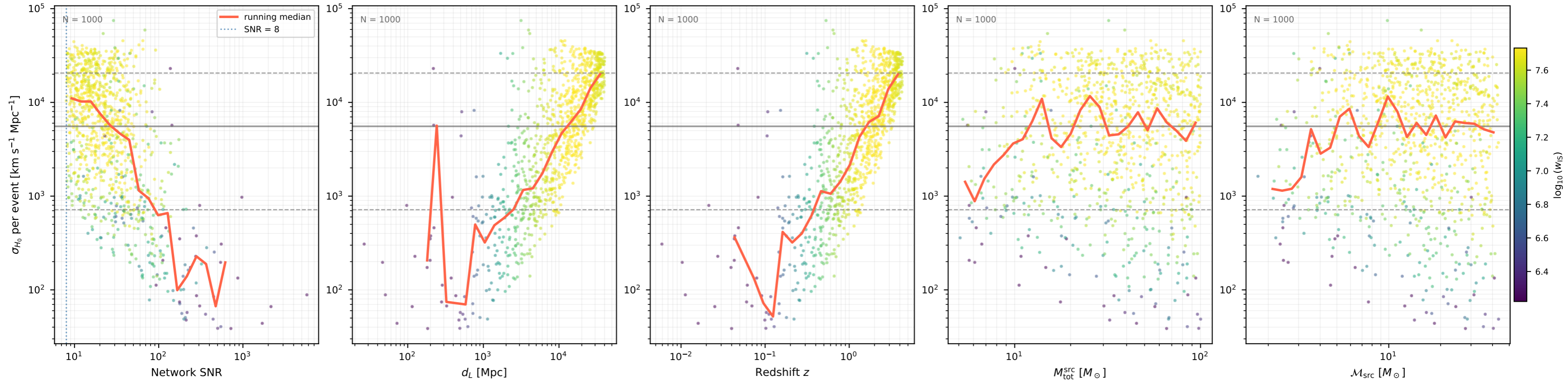
Fisher \sigma_{H_0} per event var03 (1000 events, 10 seed(s))
