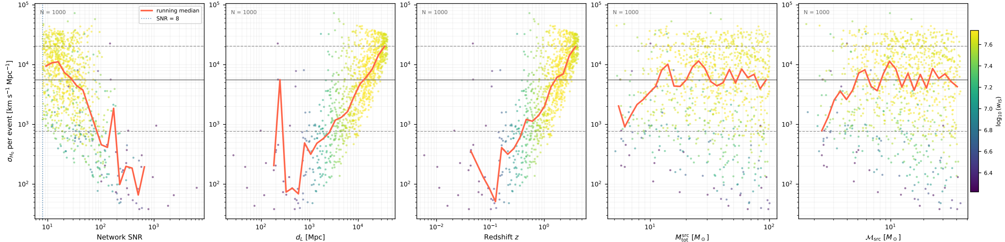
Fisher \sigma_{H_0} per event var02 (1000 events, 10 seed(s))
