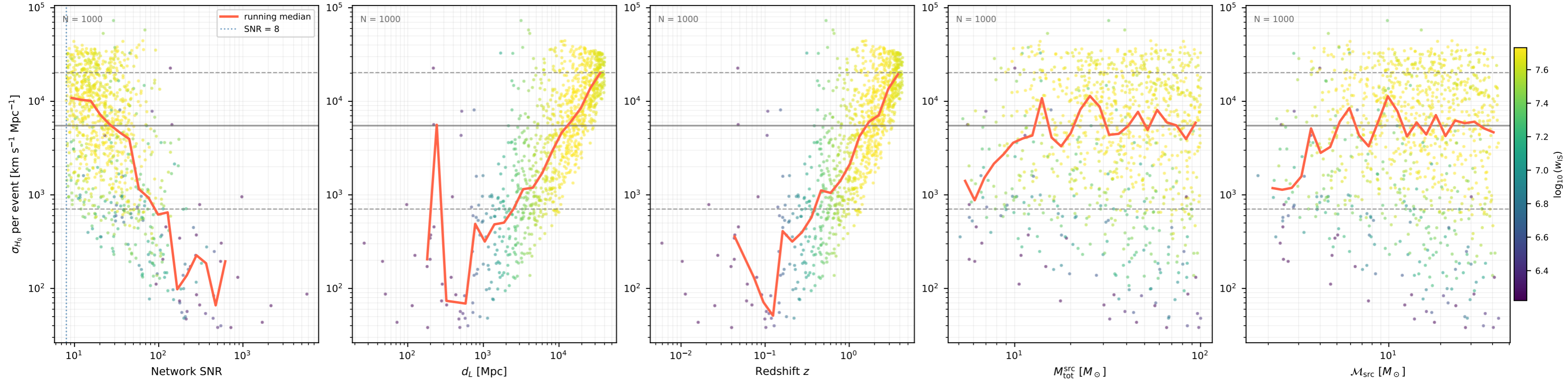
Fisher \sigma_{H_0} per event baseline (1000 events, 10 seed(s))
