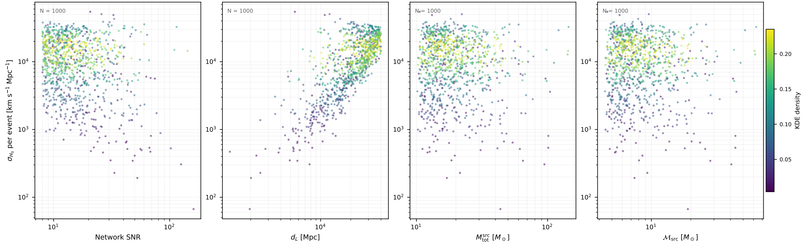
Fisher \sigma_{H_0} per event ET / var08 (1000 events, 10 seed(s))
