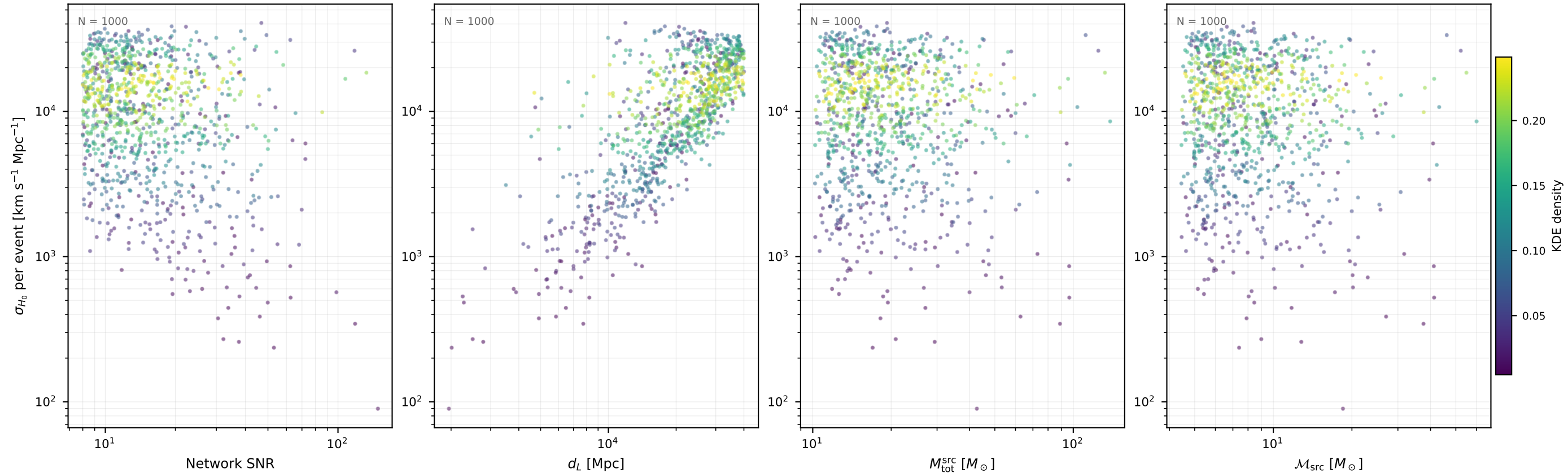
Fisher \sigma_{H_0} per event ET / var07 (1000 events, 10 seed(s))
