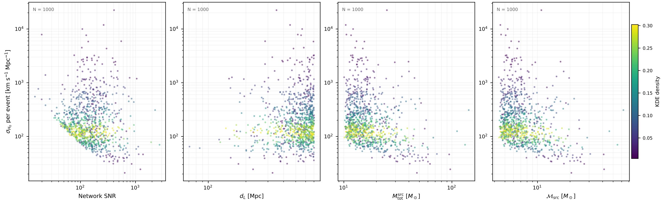
Fisher \sigma_{H_0} per event ET / dLnear700 (1000 events, 10 seed(s))
