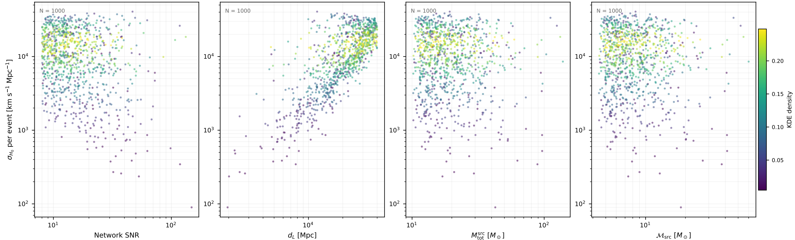
Fisher \sigma_{H_0} per event ET / baseline (1000 events, 10 seed(s))
