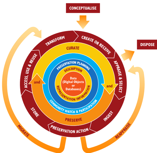
Figure 6: The DCC lifecycle model, from [25]
