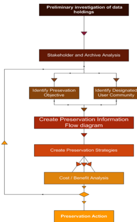
Figure 4: Preservation analysis workflow, from [19]
