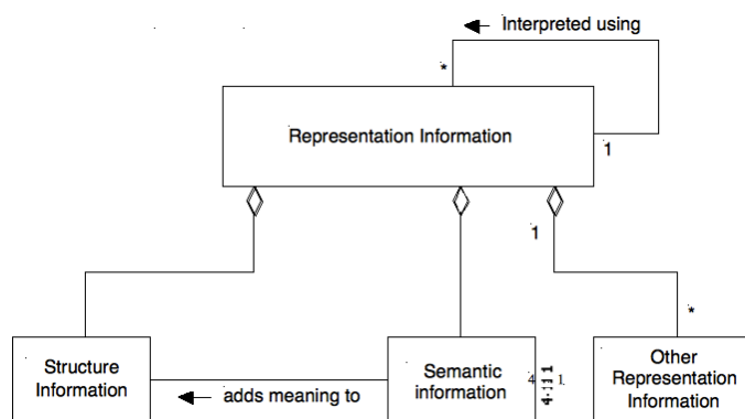
Figure 3: Representation Information Object
