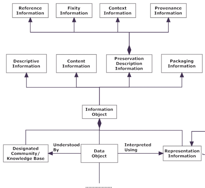
Figure 1: The OAIS information model
