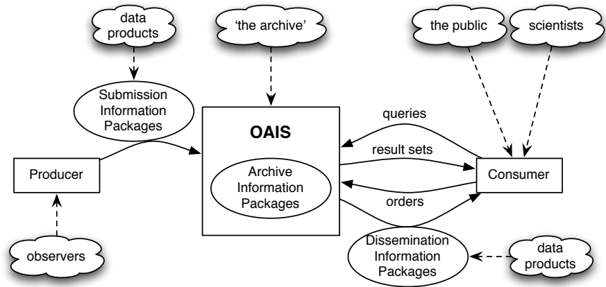
Figure 2: The highest-level structure of an OAIS archive, annotated with the corresponding labels from conventional astronomical practice (redrawn from [1, Fig. 2-4]). The dissemination data products will often in practice be the same as the submitted ones, but archives can sometimes create value-added ones of their own.
