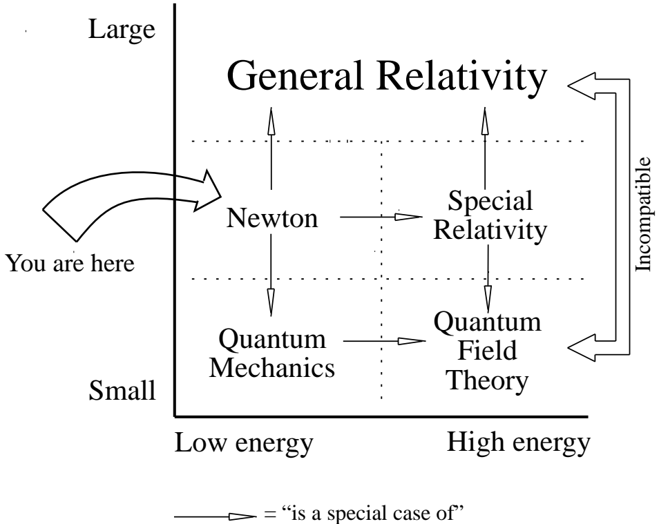
Figure 1: Physics covers a huge range of situations from very large to very small scales, and from (normal) small energies to the very large. This diagram shows how different physical theories cover different areas of this range.
